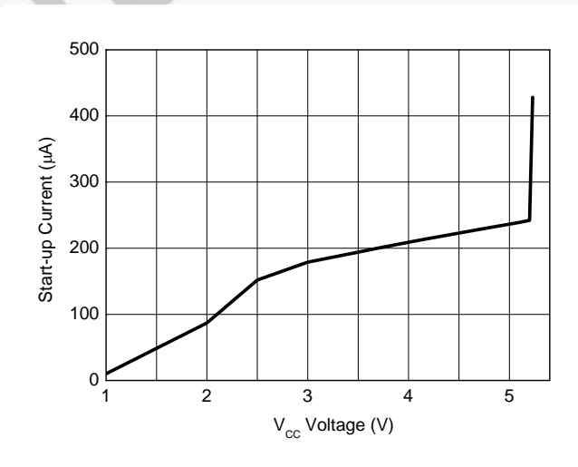
Figure 7. Start-up Current vs. V CC Voltage
