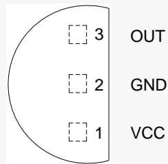
Figure 2. Pin Configuration of AP3700E (Top View)
