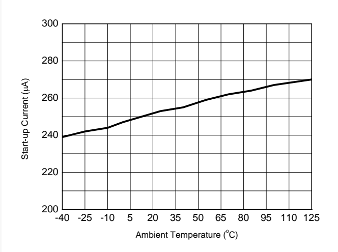
Figure 5. Start-up Current vs. Ambient Temperature
