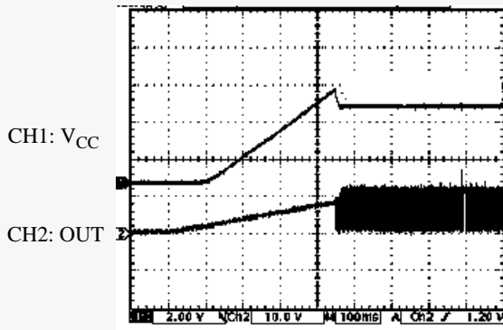
Figure 9. Start-up Sequence of V CC and V OUT
