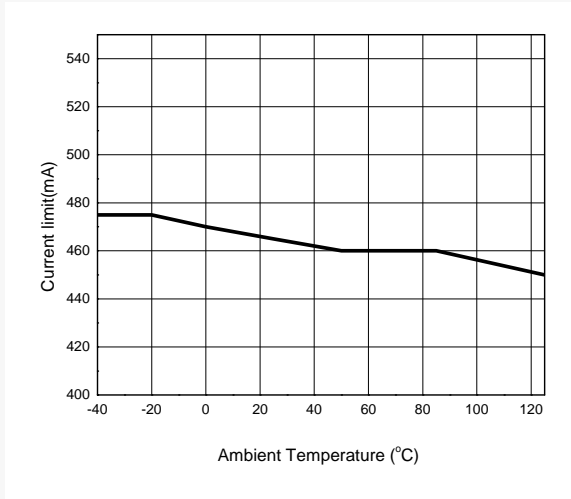
Figure 8. Current Limit vs. Ambient Temperature
