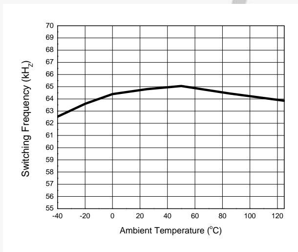
Figure 6. Switching Frequency vs. Ambient Temperature
