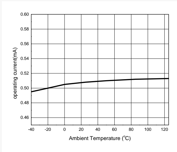
Figure 4. Operating Current vs. Ambient Temperature
